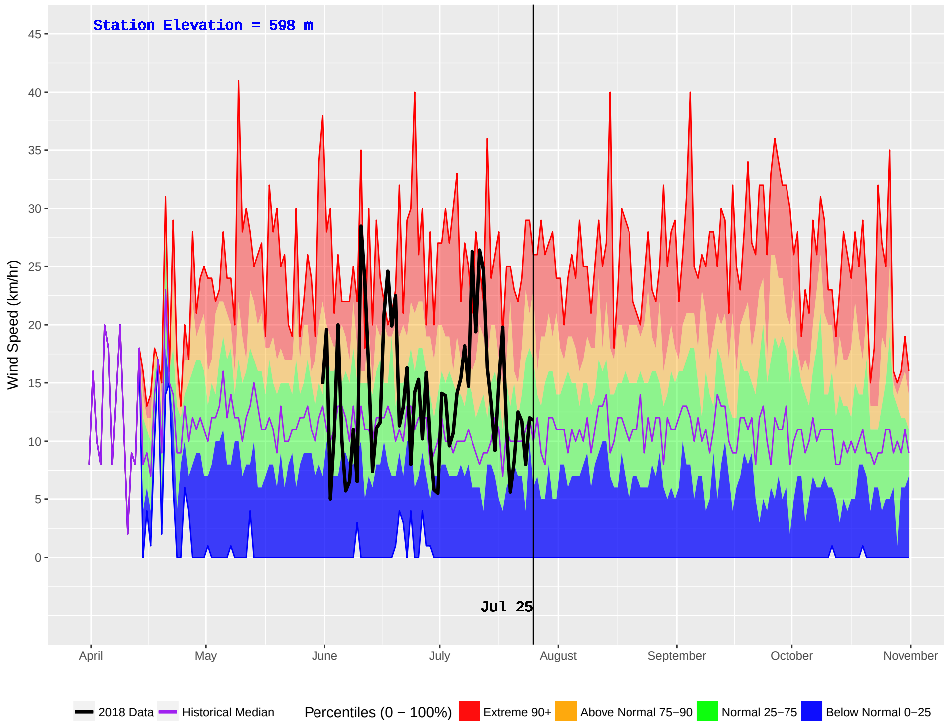
HELMUT (118) : Historical (1983–2016) and Current (2018) Noon Wind Speed
