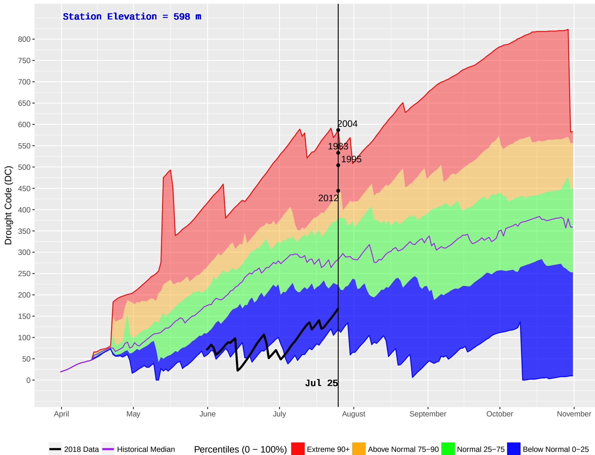
HELMUT (118) : Historical (1983–2016) and Current (2018) Noon Drought Code (DC)
